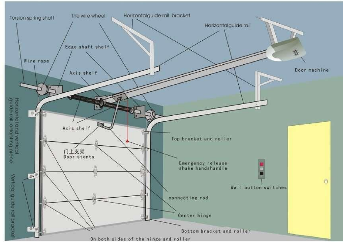
Accessories of garage door
