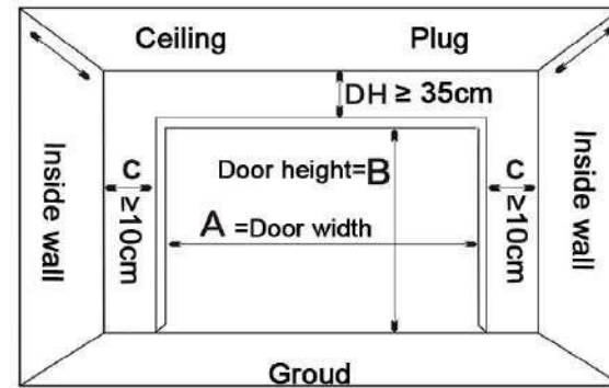
Installation space requirement
