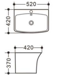
9507 520*420*370mm - Wall-hung Basin Wall-hung Installation
